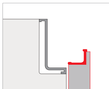
ANTA CON PROFILO AD "L" (OPZ. PL + COD. COLORE) DOOR WITH "L" SHAPED PROFILE
